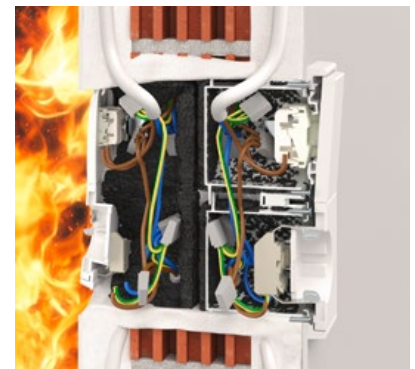
Minimum remaining wall thickness \leq 60 mm
