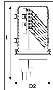
FDN 59 Port A-Length Ribbon Closure
