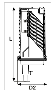
FDN 59 Port AB-Length Closure with Basket
