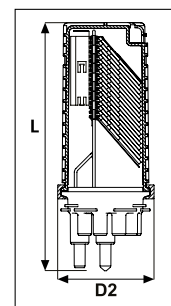
FDN 16 Port Base AB-Length Closure with Basket
