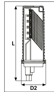
FDN 59 Port B-Length Closure with Basket
