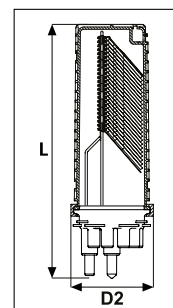
FDN 16 Port Base B-Length Closure
