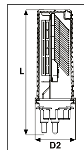
FDN 16 Port Base B-Length Closure with Basket
