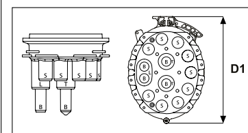
FDN 16 Port Base Configuration
