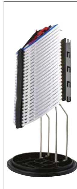
FDN 59 Port B-Length Closure with Basket
