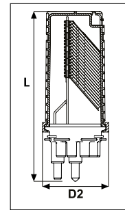
FDN 16 Port Base AB-Length Closure
