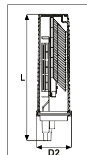
FDN IR 59 Port C-Length Closure with Basket
