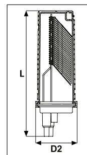
FDN 59 Port B-Length Closure
