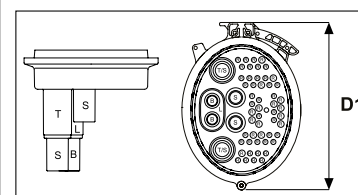
FDN 59 Port Base Port Configuration
