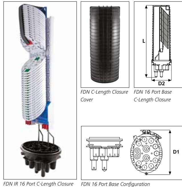
FDN IR 16 Port C-Length Closure
