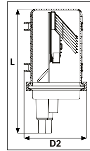
FDN IR 59 Port A-Length Closure
