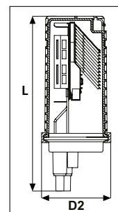
FDN IR 59 Port AB-Length Closure with Basket
