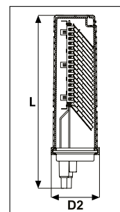
FDN 59 Port C-Length Ribbon Closure
