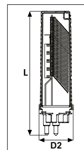
FDN 16 Port Base C-Length Closure with Basket
