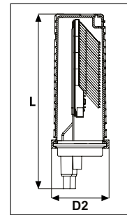
FDN IR 59 Port B-Length Closure
