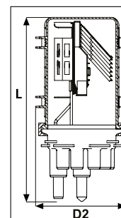
FDN 16 Port Base A-Length Closure with Basket
