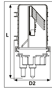
FDN 16 Port Base A-Length Closure
