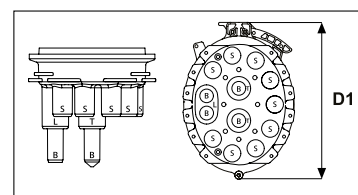
FDN 16 Port Base Configuration with Basket
