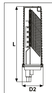
FDN 59 Port C-Length Closure with Basket
