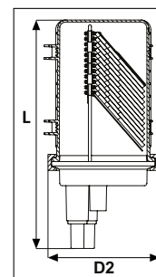
FDN 59 Port A-Length Closure
