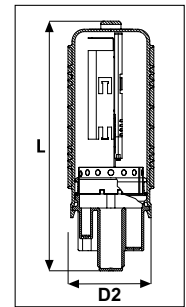
FST 13 Port with 1 Hellapon Small Tray and Basket
