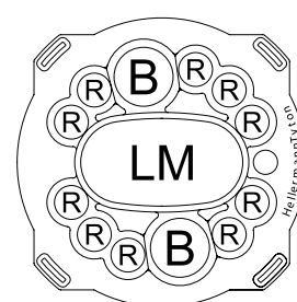
FST 13 Port Base Configuration (Cablelok only)
